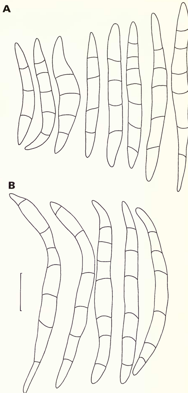
Fig. 67 Ascospore outlines (A) Porina borrieri (Trevisan) D. Hawksw. & James (Concarneau—holotype of Verrucaria longispora ); (B) Capronia longonigra (Norman) Aguirre (UPS—holotype); scale = 10 µm.
